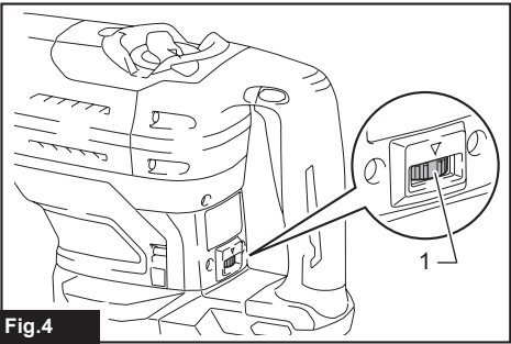
Fig.4 ► 1. Adjusting dial
