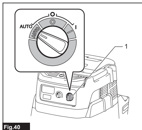
Fig.40 ► 1. Stand-by switch
